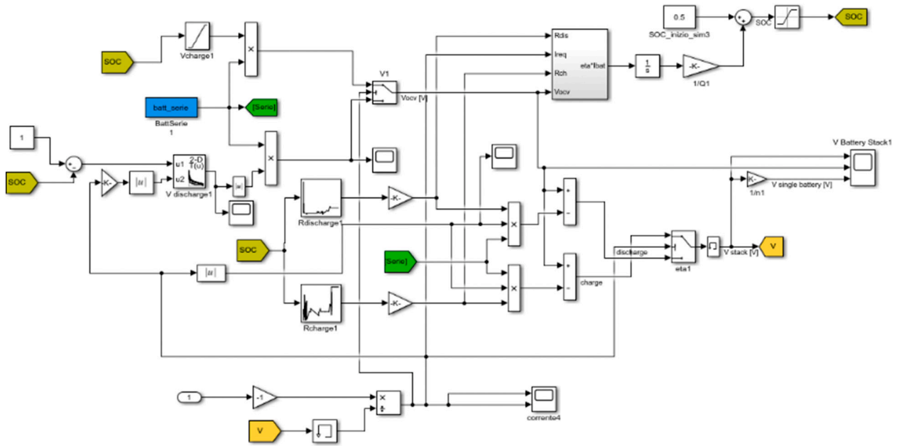
Fig. 7. Li-ion battery subsystem implementation.
